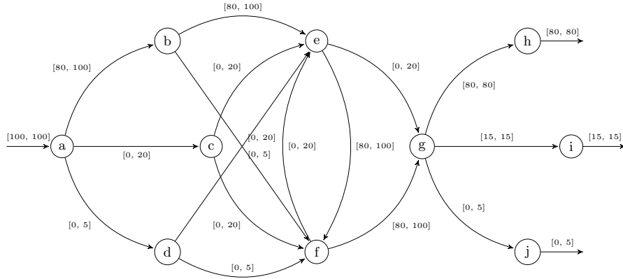
Fig. 4: The Uncertain Directly-Follows Graph (UDFG) computed based on the uncertain event log \langle a, b, e, f, g, h \rangle^{80} , \langle a, \{b, c\}, [e, f], g, i \rangle^{15} , \langle a, \{b, c, d\}, [e, f], g, \bar{j} \rangle^5 . The arcs are labeled with the minimum and maximum number of directly-follows relationship observable between activities in the corresponding trace. Notice the large amount of connections extracted from a single and rather short trace. Uncertain directly-follows relationships are inferred from the behavior graphs of the traces in the log. The construction of this object is necessary to perform automatic process discovery over uncertain event data.
