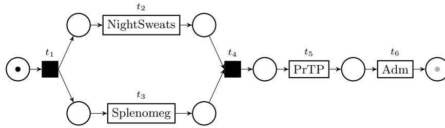
Fig. 2: A normative model for the healthcare process case in the running example. The initial marking is displayed; the gray “token slot” represents the final marking.
