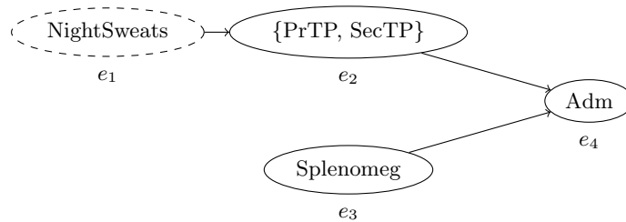
Fig. 1: The behavior graph of the trace in Table 1. Every node represents an event; the labels in the nodes represent the activity, or set of activities, associated with the event. The arcs represent the partial order relationship between events as defined by their timestamps. The indeterminate event, which might not have occurred, is represented by a dashed node.
