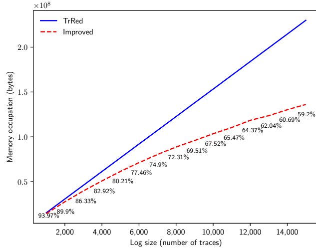
Fig. 14: Memory consumption in bytes needed to store the behavior graphs for synthetic uncertain event logs with traces of length l = 10 events and timestamp uncertainty of p = 0.5 , with an increasing number of traces n .
