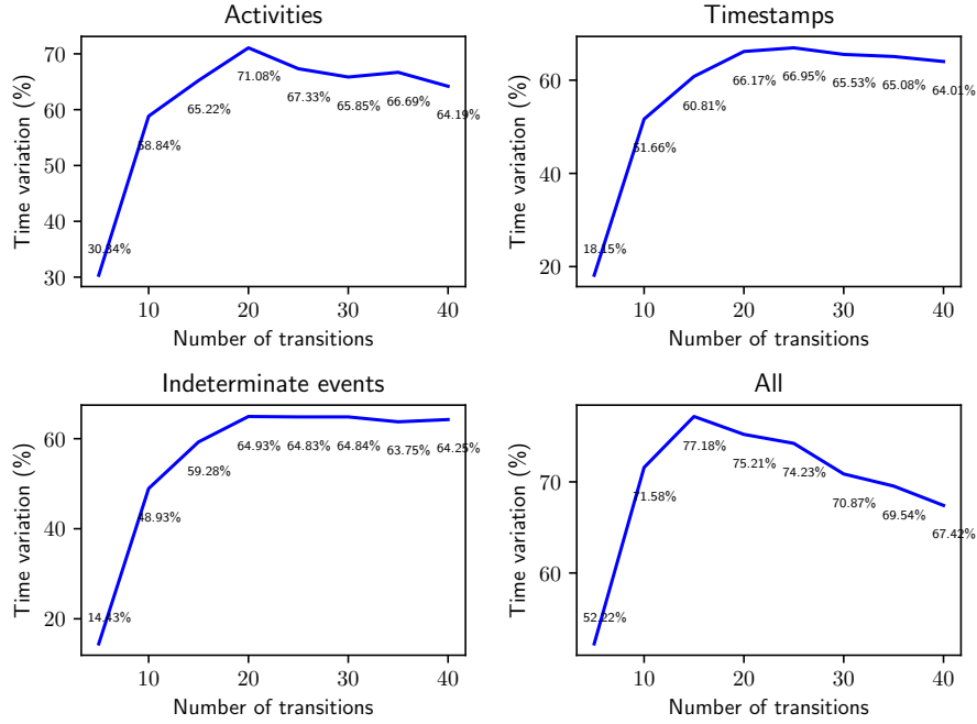
Fig. 16: Relative variation in computation time obtained through the improved behavior graph construction when applied to the computation of conformance bounds between a synthetic uncertain log and a Petri net with an increasing number of transitions. The synthetic uncertain logs have n = 500 traces and timestamp uncertainty has been introduced with p = 0.1 .
