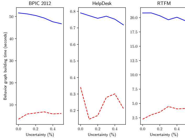
Fig. 15: Execution times in seconds for real-life event logs with increasing percentages p of timestamp uncertainty.
