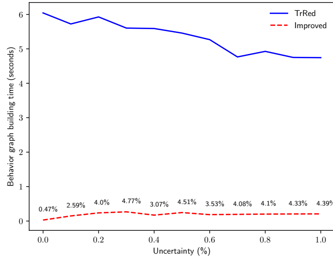
Fig. 13: Time in seconds for the creation of the behavior graphs for synthetic logs with n = 100 traces of length l = 100 events, with increasing percentages of timestamp uncertainty p .
