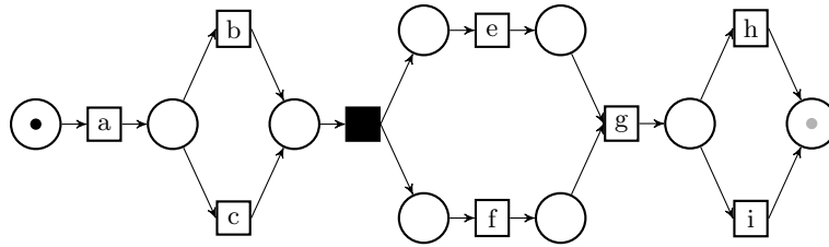
(b) A process model that can replay some – but not all – the relationships appearing in the uncertain parts of the traces in the uncertain log. This process model mediates between representing only certain observation and representing all the possible behavior in the process.
