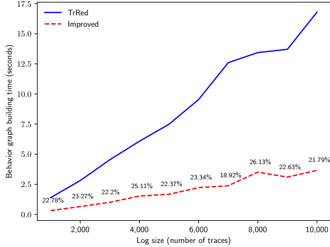
Fig. 11: Time in seconds for the creation of the behavior graphs for synthetic logs with traces of length l = 20 events and p = 0.5 of uncertain events, with increasing number of traces n . The solid blue line indicates the time needed for the naïve construction; the dashed red line shows the building time of the improved algorithm, and is labeled with the relative time variation (in percentage).
