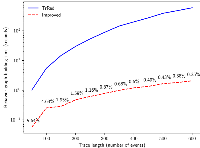
Fig. 12: Time in seconds for the creation of the behavior graphs for synthetic logs with n = 100 traces and p = 0.5 of uncertain events, with increasing trace length l .
