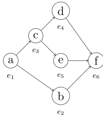
Fig. 9: The behavior graph of the trace in Table 4.
