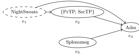
Fig. 6: The behavior graph of the trace in Table 1 before applying the transitive reduction. All the nodes in the graph are pairwise connected based on precedence relationships; pairs of nodes for which the order is unknown are not connected.
