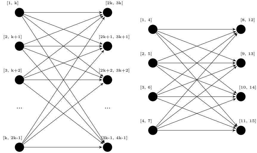
Fig. 10: Construction of the class of behavior graphs isomorphic to a complete bipartite graph and an instantiated example. For any n = 2k , it is possible to have a behavior graph isomorphic to the graph K_{k,k} , which thus has a number of edges quadratic in the number of vertices.
