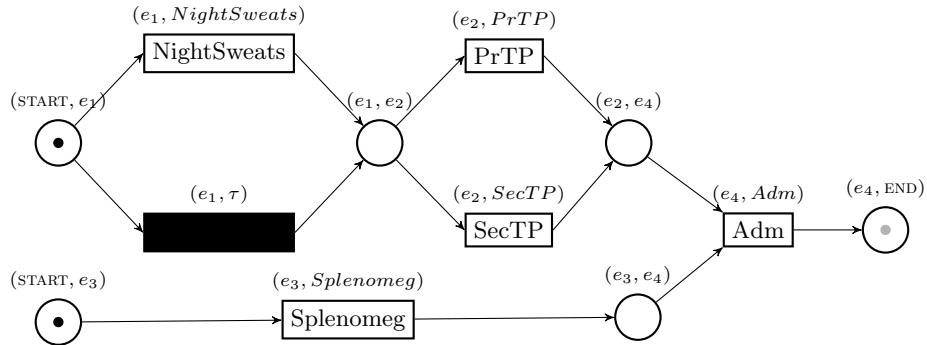
Fig. 3: The behavior net representing the behavior of the uncertain trace in Table 1 and obtained thanks to its behavior graph. The initial marking is displayed; the gray “token slot” represents the final marking. This artifact is necessary to perform conformance checking between uncertain traces and a reference model.
