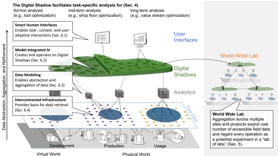
Fig. 2. In the Internet of Production (IoP), task-adaptive Digital Shadows build on interconnected infrastructure, data modeling, and model-integrated artificial intelligence to provide smart interfaces that make the right data actionable at the right time during development, production, and usage. Integration across different production facilities and locations leads to the World Wide Lab.
