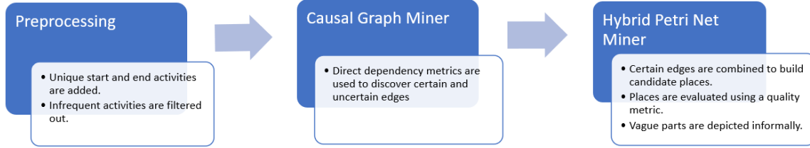
Fig. 3: Three steps of the hybrid Miner.
