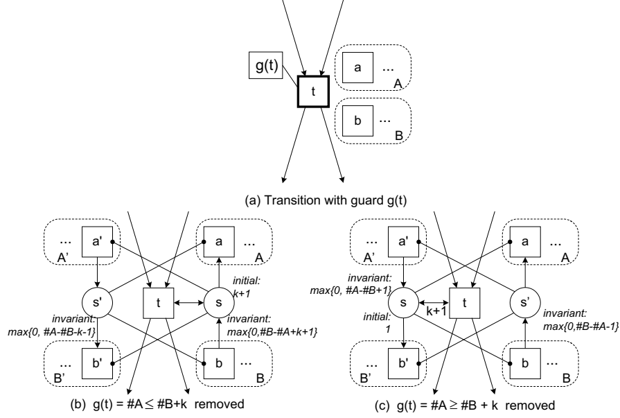
Fig. 5. Replace the guard by places s and s' , duplicate transitions, and inhibitor arcs.
