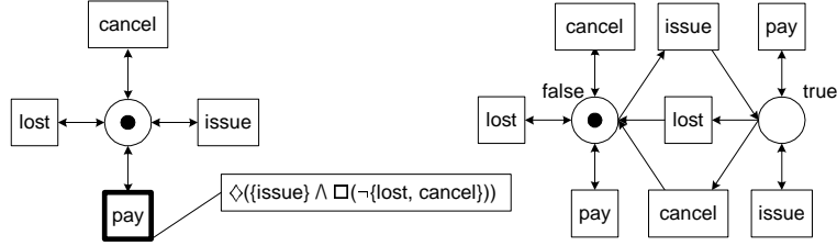
Fig. 8. A net with an LTL-guard
