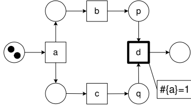
Fig. 3. A token history net.
