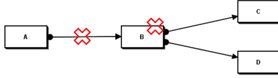
Fig. 8. Implicit constraints between A and C and between A and D are omissible
