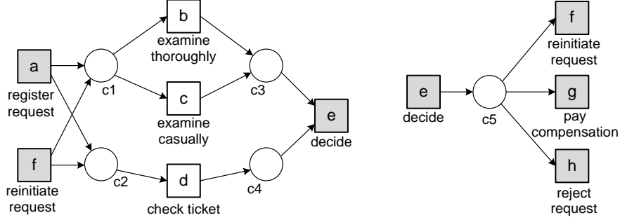
Figure 6. Two net fragments corresponding to the two passages of the skeleton in Fig. 5: PN_1 = PN^{\{\{a,f\},\{e\}\}} (left) and PN_2 = PN^{\{\{e\},\{f,g,h\}\}} (right). The visible transitions T_v = \{a, e, f, g, h\} that form the boundaries of the fragments are highlighted.
