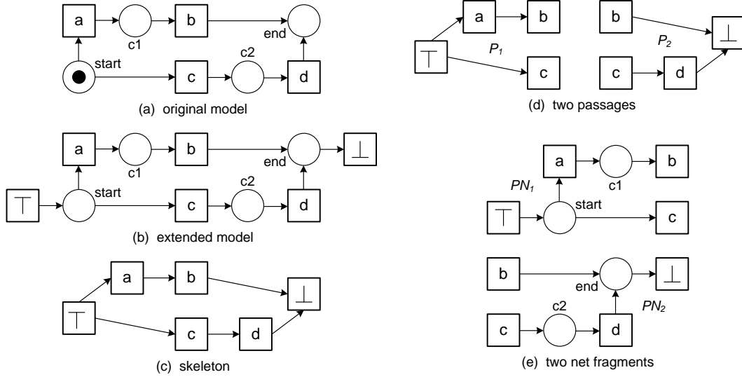
Figure 8. The system net SN = (PN, [start], [end]) shown in (a) is extended into system net \overline{SN} = (\overline{PN}, [], []) by adding artificial start ( \top ) and complete ( \perp ) transitions as shown in (b). The skeleton skel(\overline{PN}) is shown in (c). A passage partitioning composed of P_1 = (\{\top, a\}, \{a, b, c\}) and P_2 = (\{b, c, d\}, \{d, \perp\}) is shown in (d) and the corresponding two net fragments are shown in (e).
